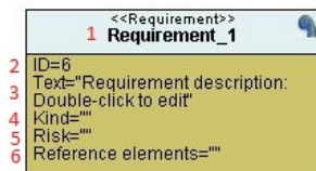
Figure 9: Requirement Box
