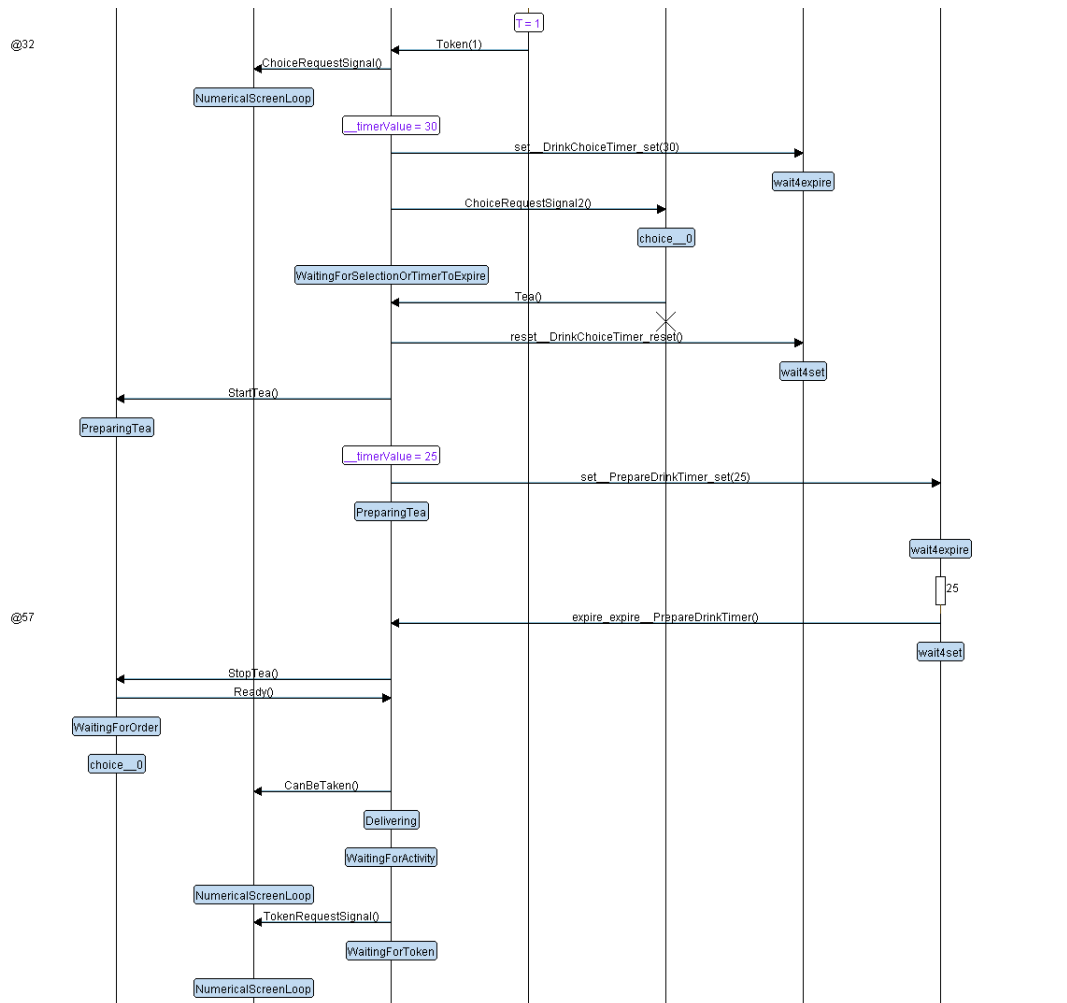
Figure 36: Simulation steps (part 2)
