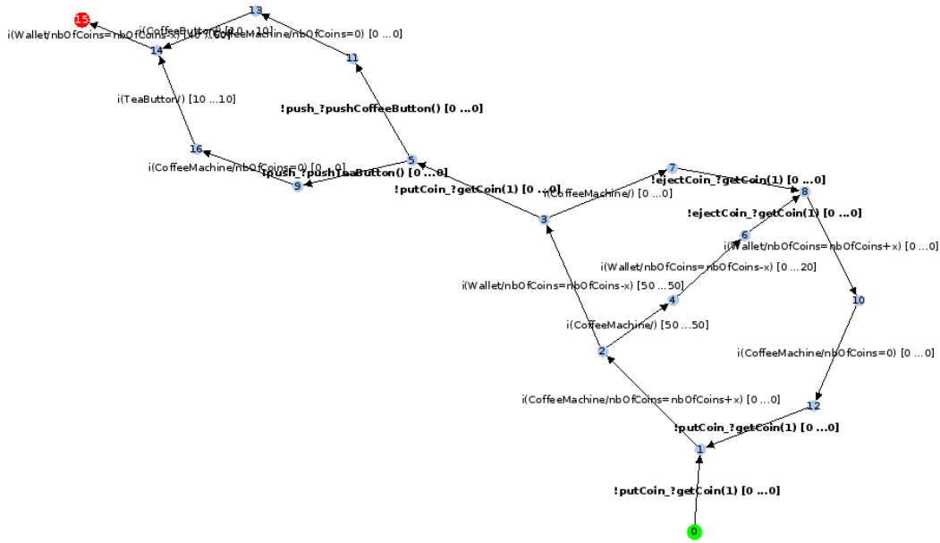
Figure 37: Reachability graph
