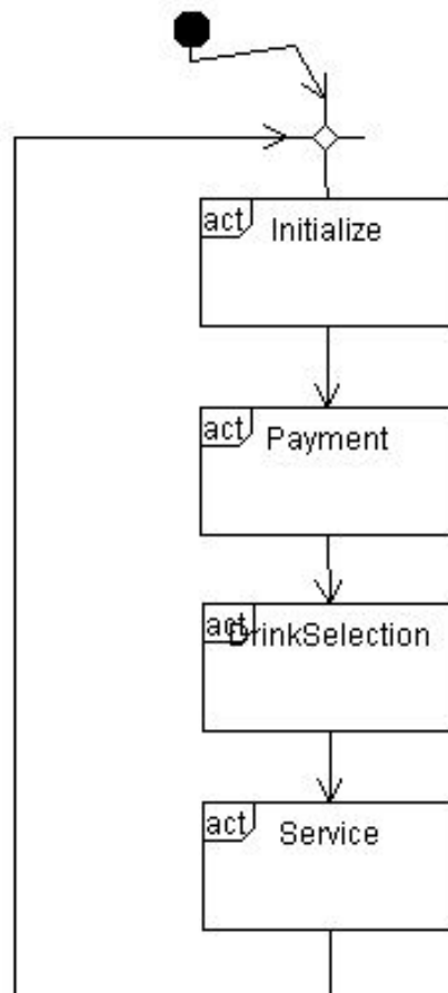
Figure 18: Activity Diagram
